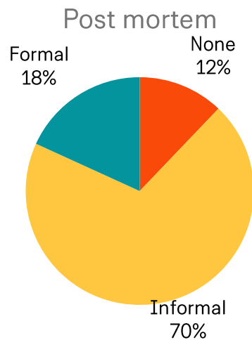
Figure 10 Postmortem
