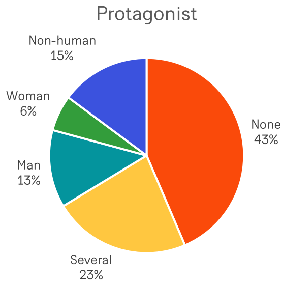
Figure 24 Protagonist type
