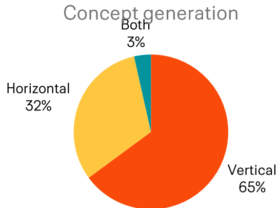
Figure 16 Concept generation
