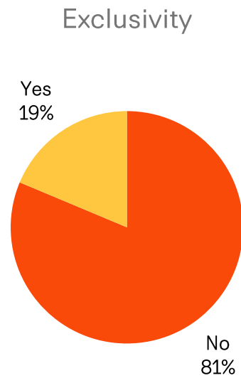
Figure 6 Exclusivity
