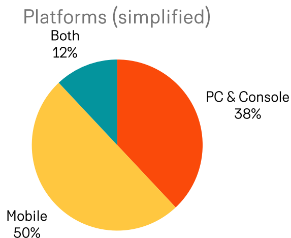
Figure 19 Platforms
